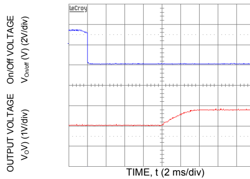
Figure 17. Typical Start-Up with Prebias ( V_{in} = 5.5\text{ Vdc} , V_o = 1.8\text{ Vdc} , I_o = 1\text{ A} , V_{bias} = 1.0\text{ Vdc} ).
