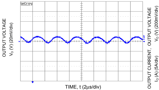
Figure 8. Typical Output Ripple and Noise ( V_{in} = 5.0V dc, V_o = 0.75 , Vdc, I_o = 10A ).
