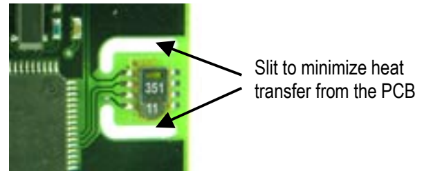
Figure 14 SHT1x PCB Mounting example
